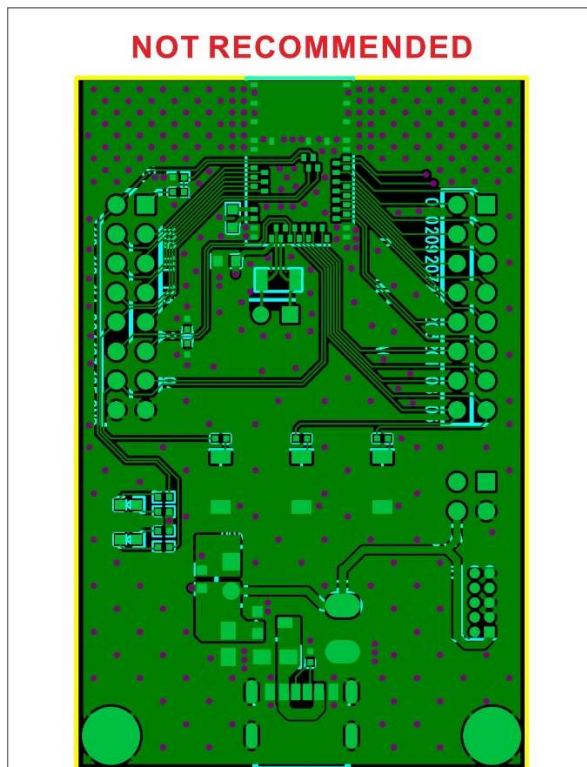
TOP VIEW
