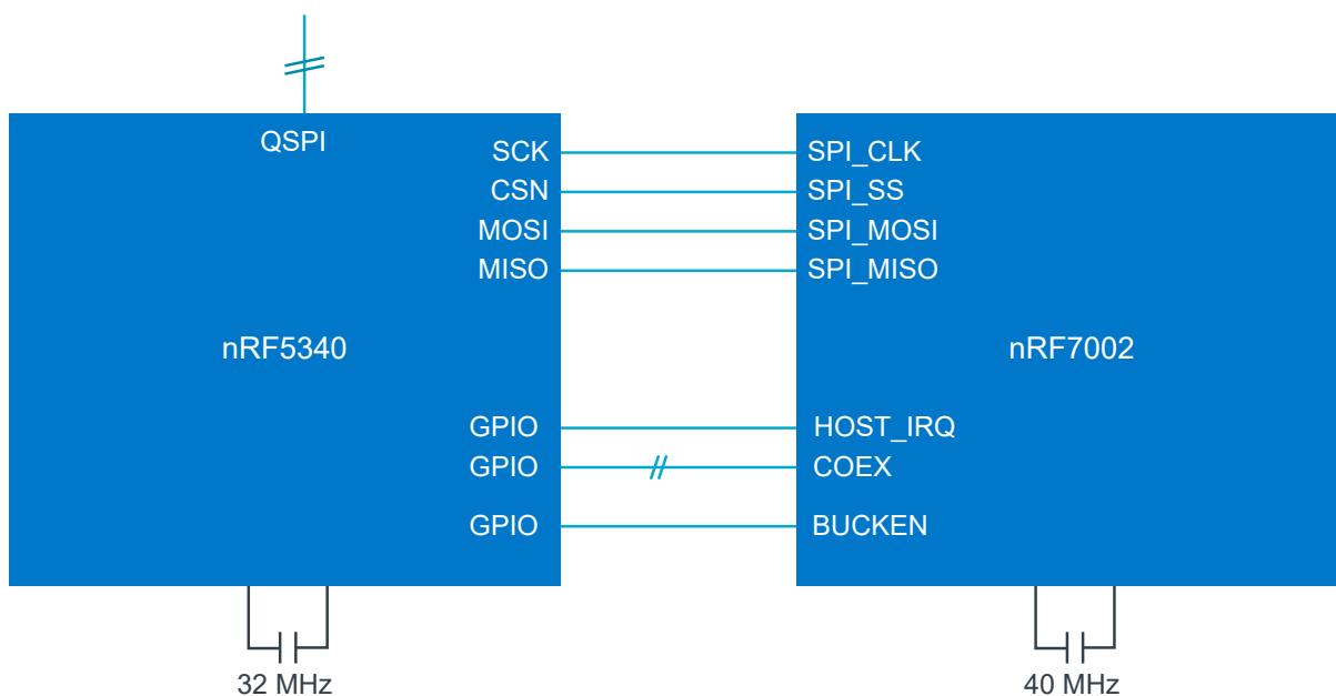
Figure 34: SPI connection
