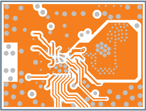
Figure 28: Mid layer 1
