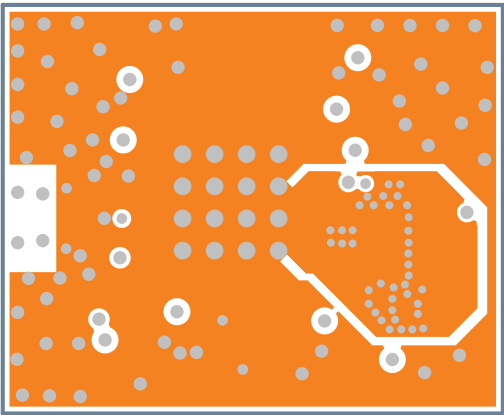
Figure 22: Mid layer 1
