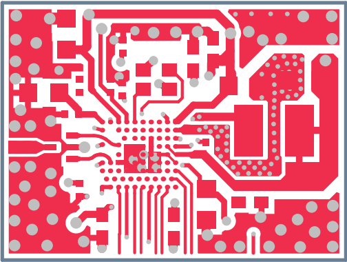
Figure 27: Top layer
