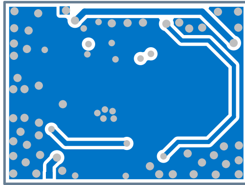
Figure 30: Bottom layer
