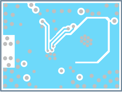
Figure 29: Mid layer 2
