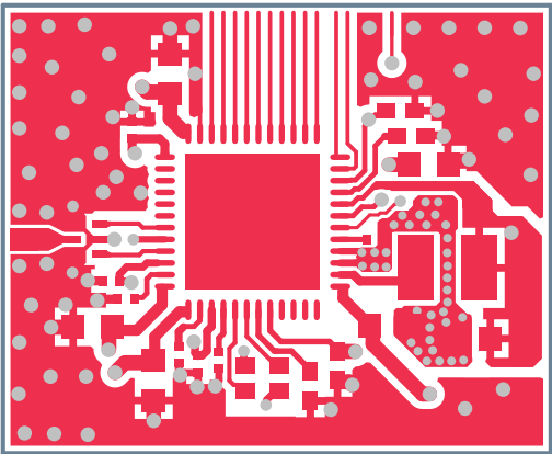
Figure 21: Top layer
