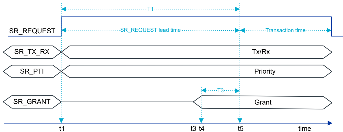
Figure 16: 4-wire timing
