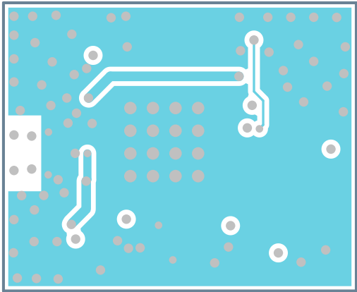
Figure 23: Mid layer 2
