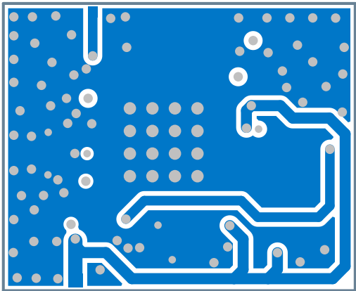
Figure 24: Bottom layer
