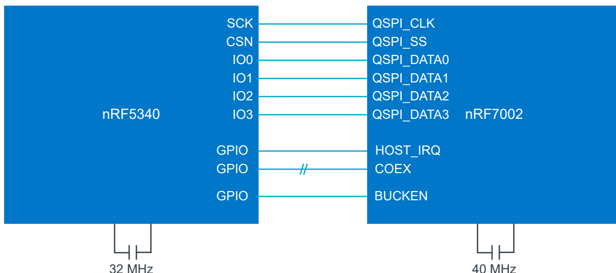
Figure 33: QSPI connection
